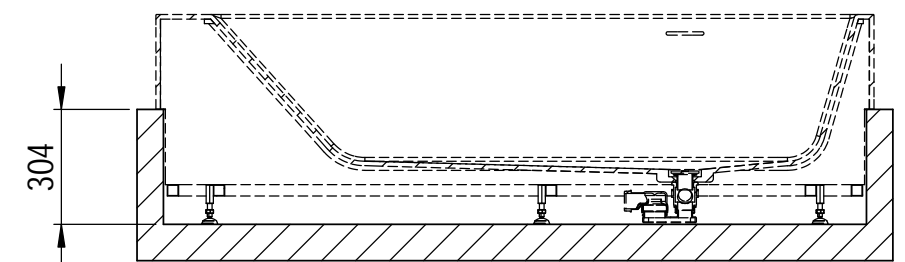
DIMENSIONI FORO PER INCASSO VASCA HOLE DIMENSIONS TO BUILT-IN THE BATHTUB
